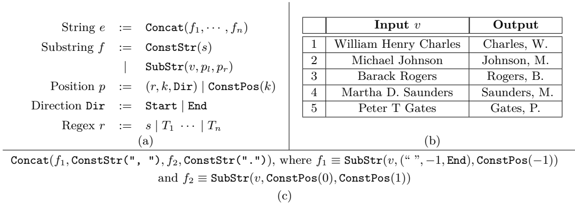
■ Figure 2 (a) The regular expression based string transformation DSL, (b) an example task in the DSL for transforming names to last names followed by first name initial, and (c) an example program in the DSL for this task.
