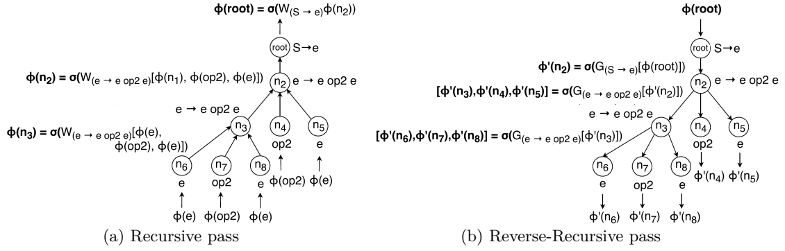
■ Figure 4 (a) The initial recursive pass of the R3NN. (b) The reverse-recursive pass of the R3NN where the input is the output of the previous recursive pass.
