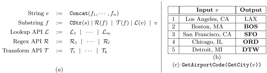
■ Figure 3 (a) The NACIO DSL for API composition, (b) a NACIO task to obtain airport code and (c) a program in the DSL for the task.
